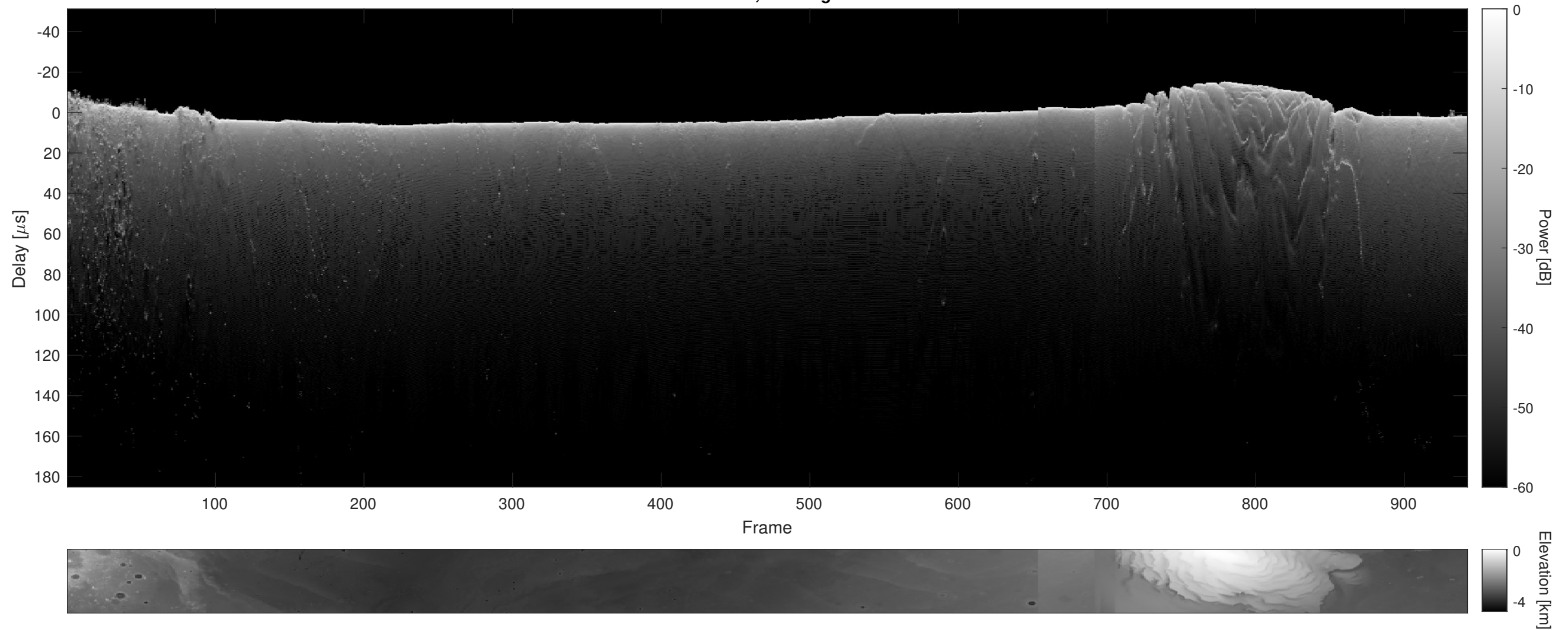
Orbit 5829, Cluttergram
