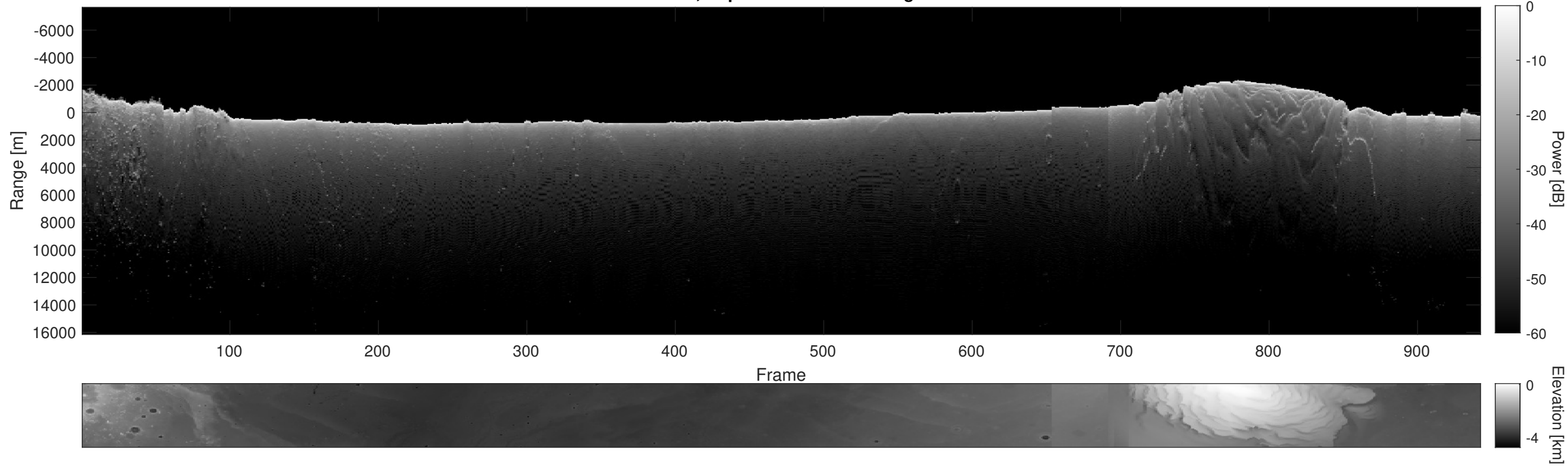
Orbit 5829, Depth-Corrected Cluttergram
