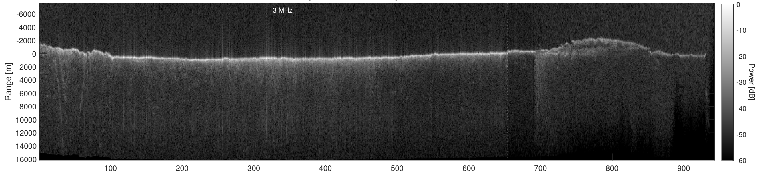
Orbit 5829, Depth-Corrected Cluttergram
