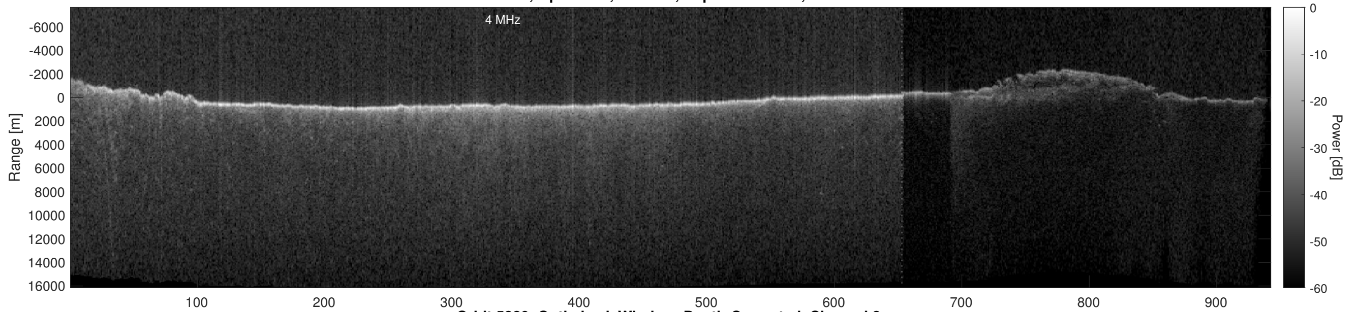
Orbit 5829, Optimized, Window, Depth-Corrected, Channel 2
