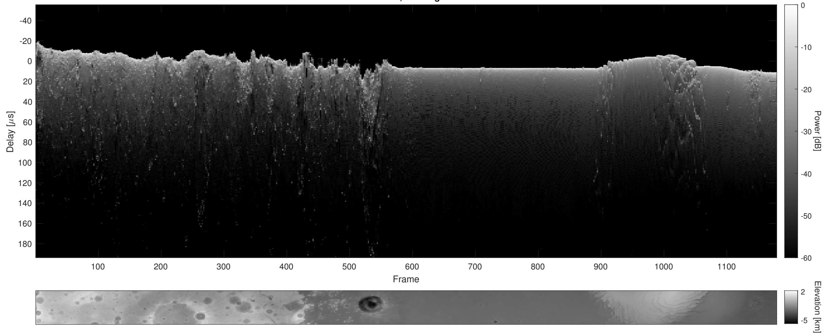
Orbit 5830, Cluttergram
