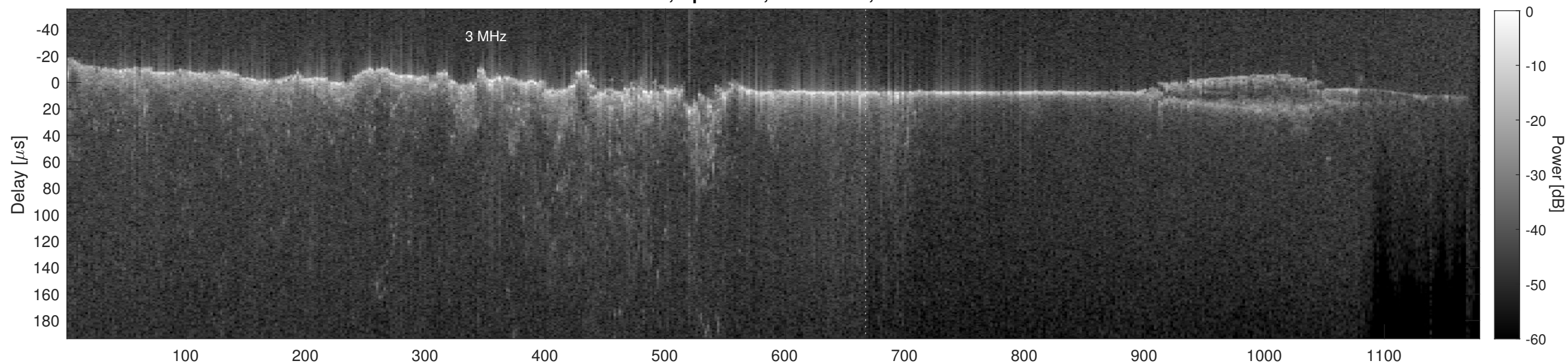
Orbit 5830, Cluttergram
