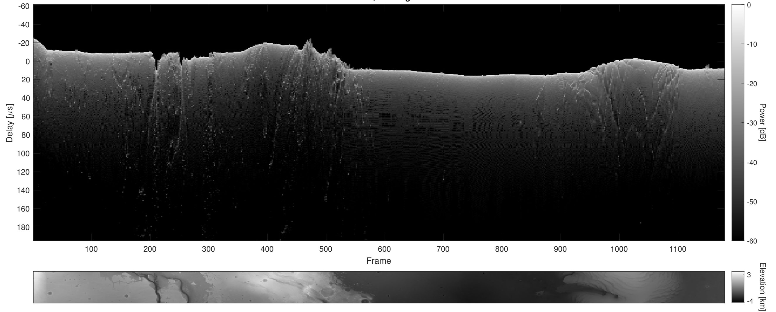
Orbit 5831, Cluttergram
