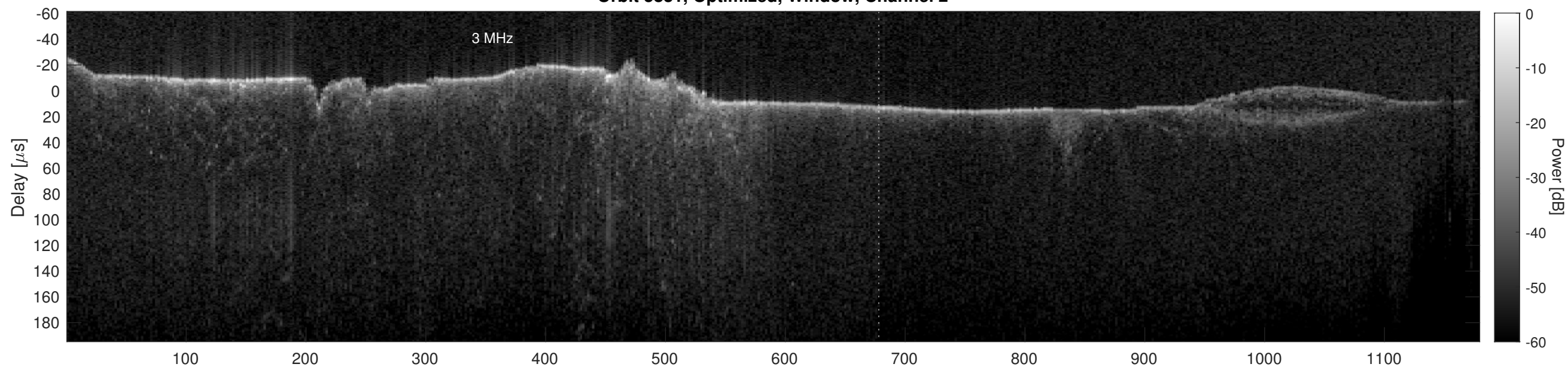
Orbit 5831, Cluttergram
