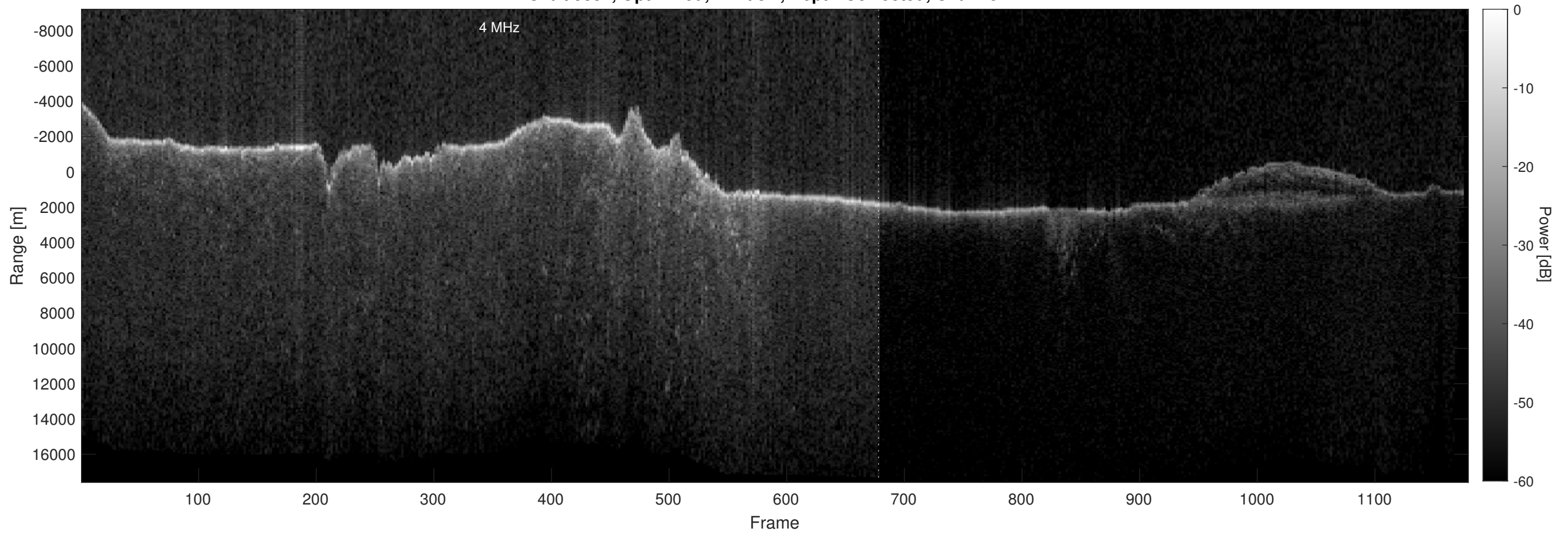
Orbit 5831, Optimized, Window, Depth-Corrected, Channel 2
