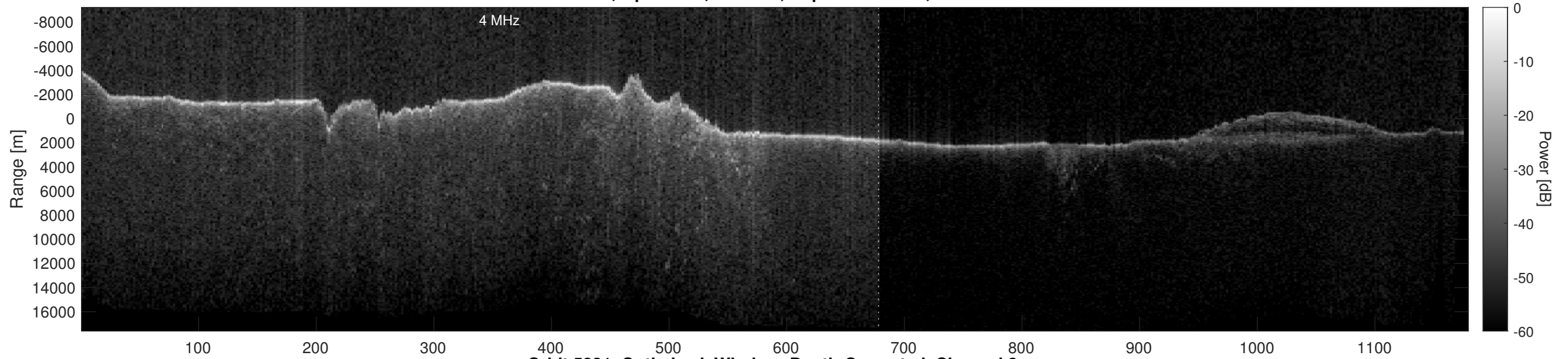
Orbit 5831, Optimized, Window, Depth-Corrected, Channel 2
