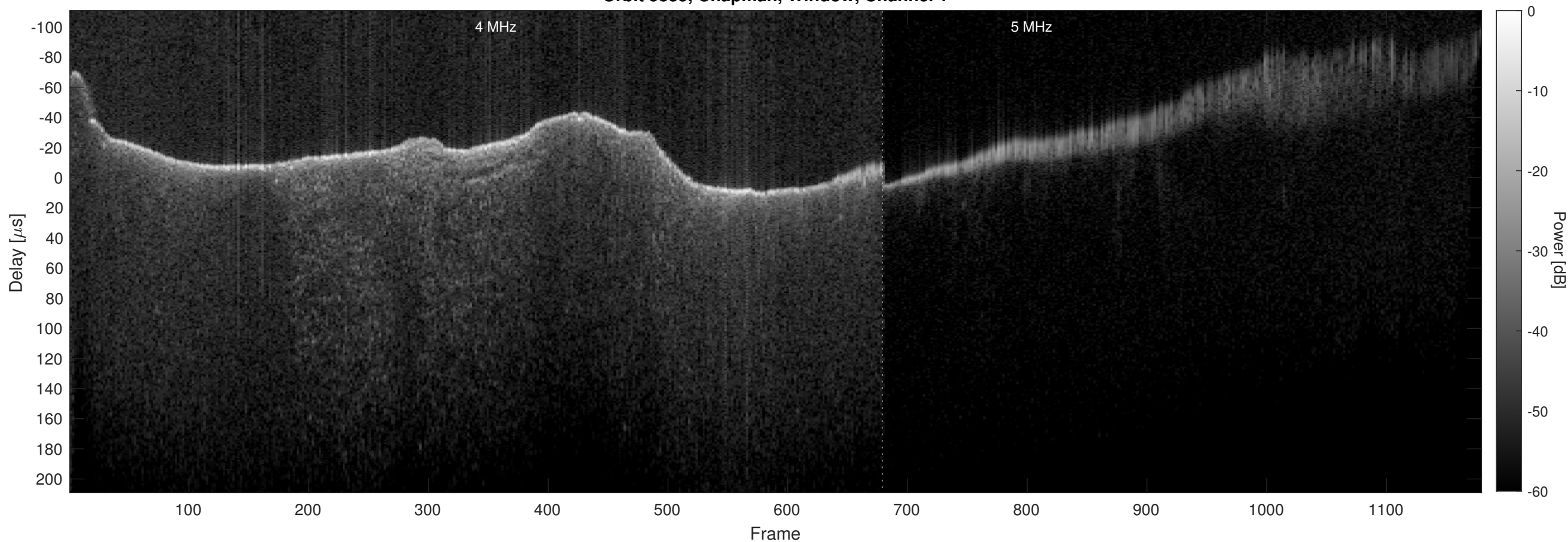
Orbit 5835, Chapman, Window, Channel 2
