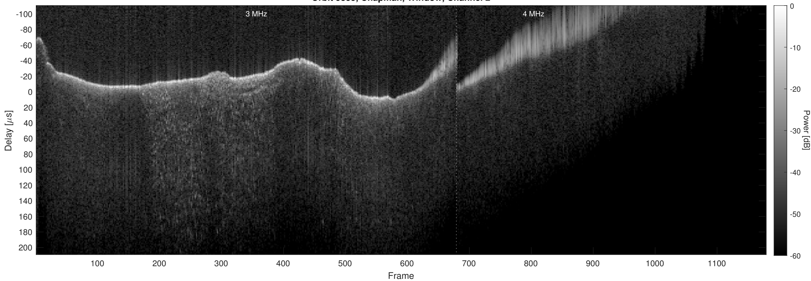
Orbit 5835, Chapman, Window, Channel 2
