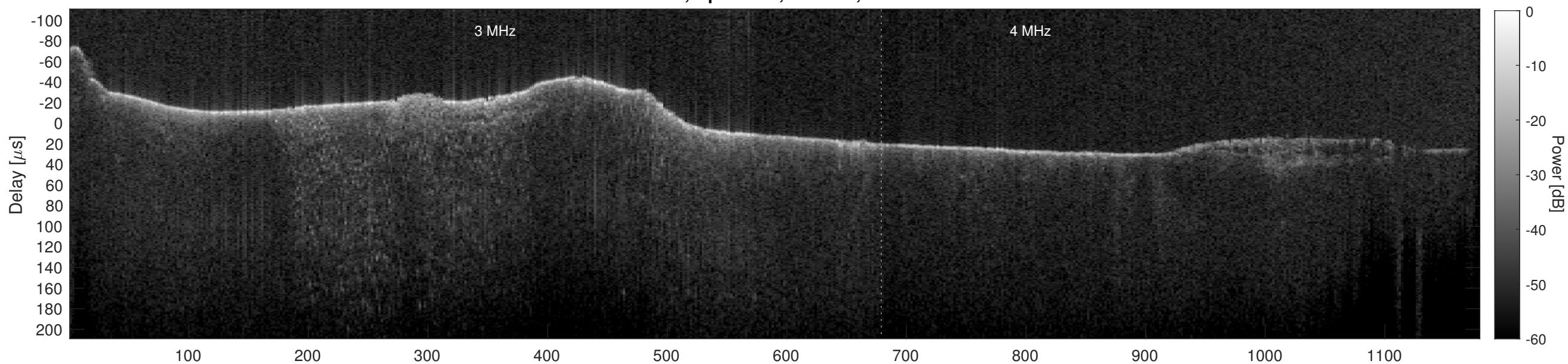
Orbit 5835, Cluttergram
