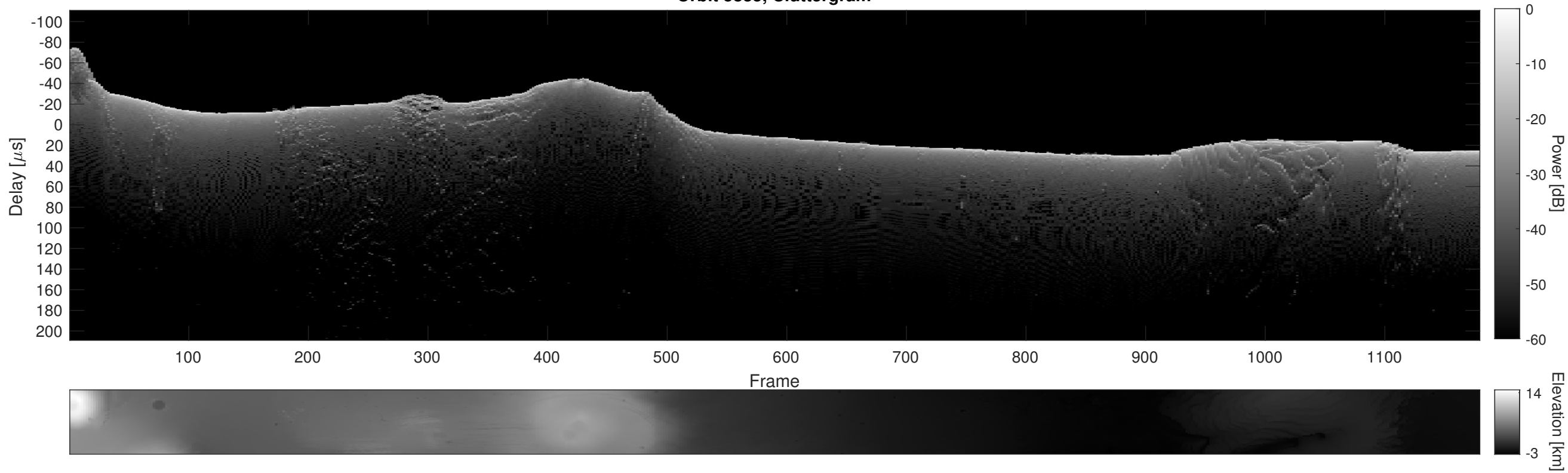
Orbit 5835, Cluttergram
