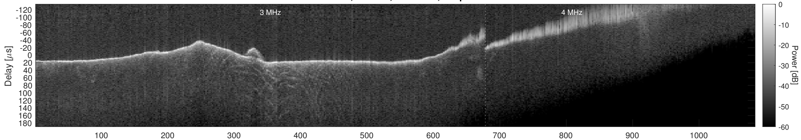
Orbit 5836, Window, Channel 2, Optimized
