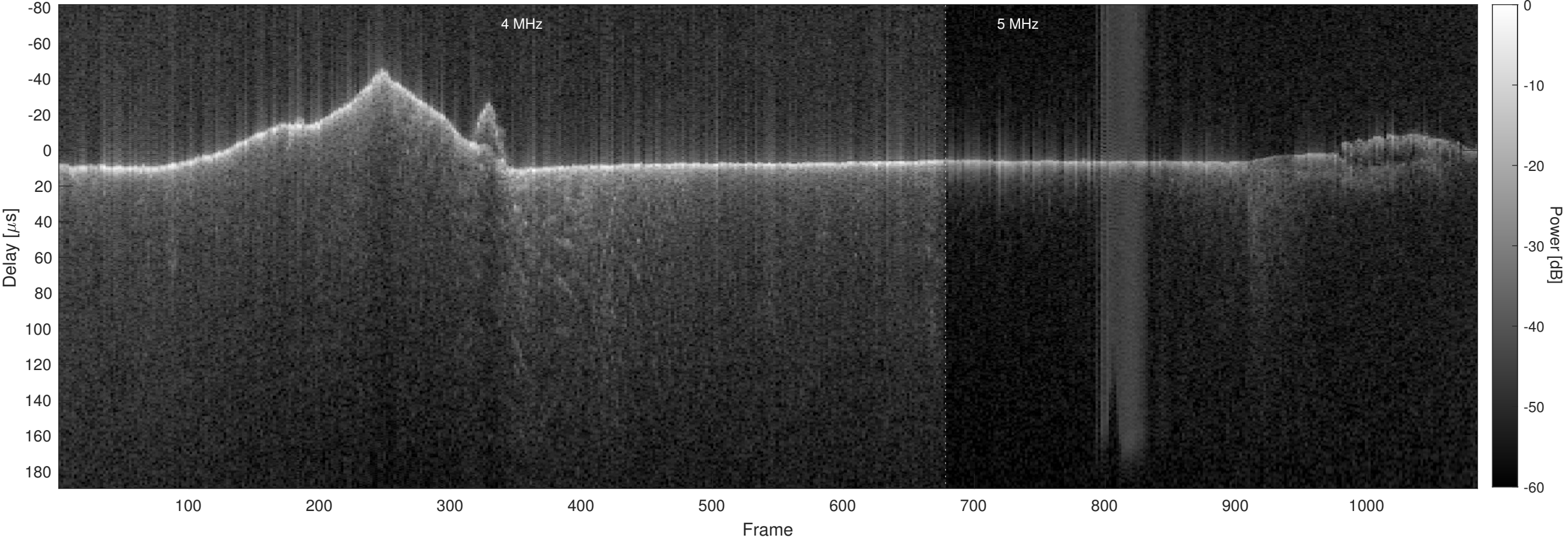
Orbit 5836, Optimized, No Window, Channel 2
