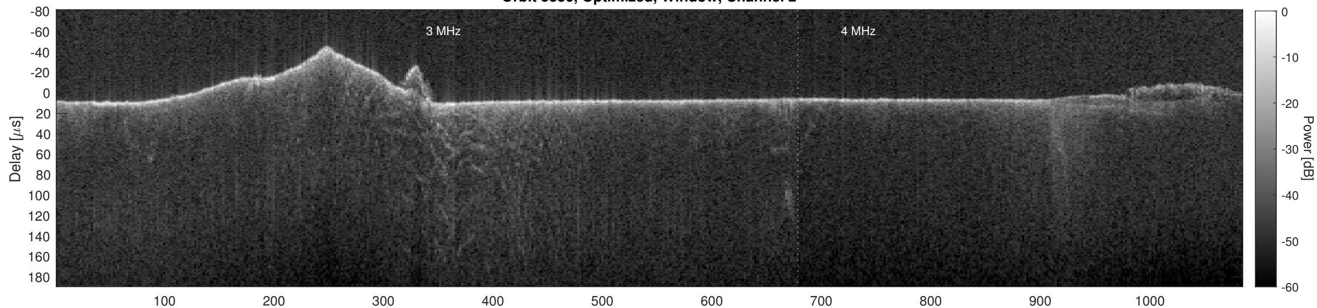
Orbit 5836, Cluttergram
