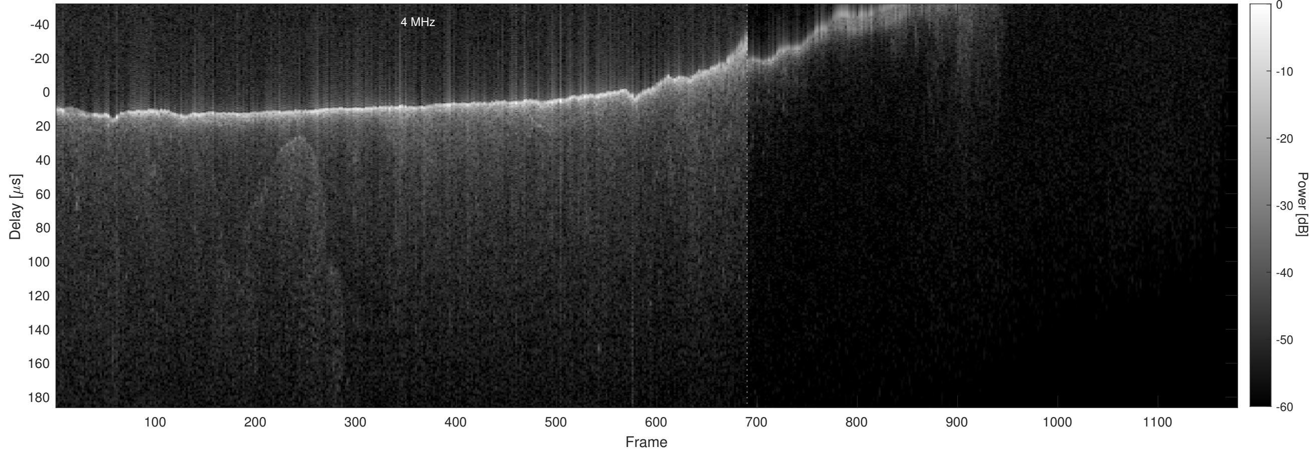
Orbit 5839, Chapman, No Window, Channel 2
