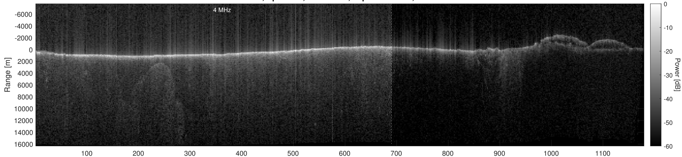
Orbit 5839, Optimized, No Window, Depth-Corrected, Channel 2
