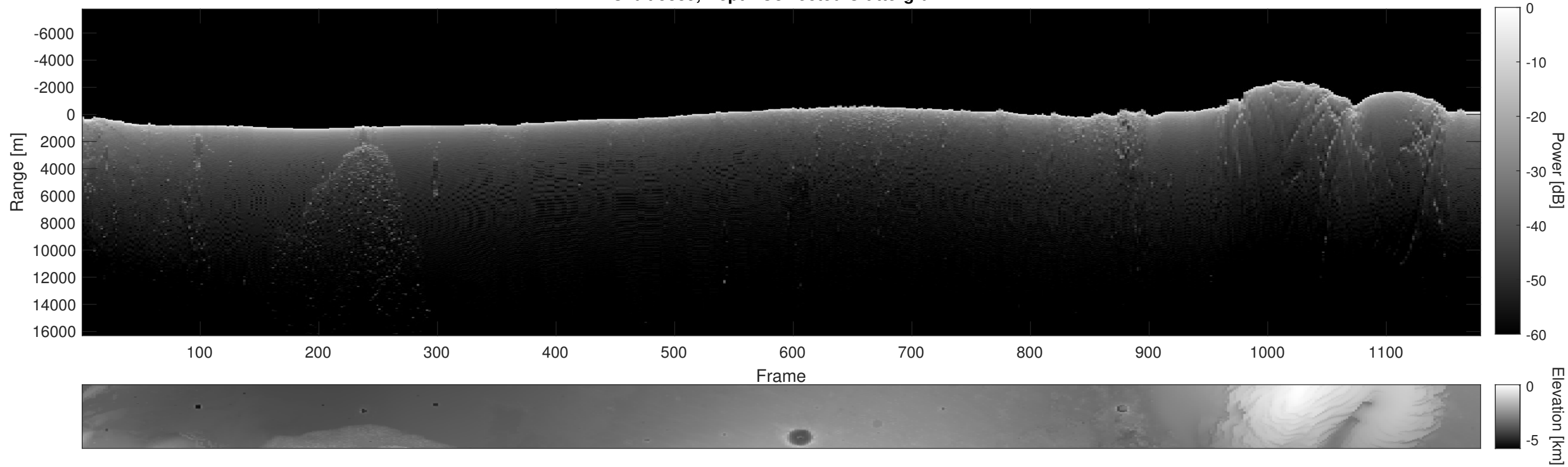
Orbit 5839, Depth-Corrected Cluttergram
