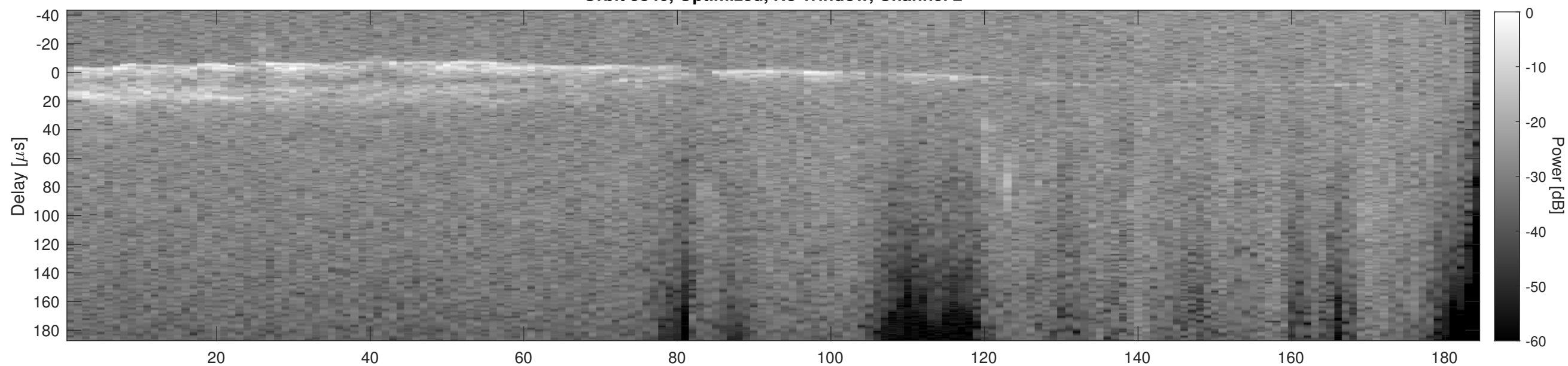
Orbit 5840, Cluttergram
