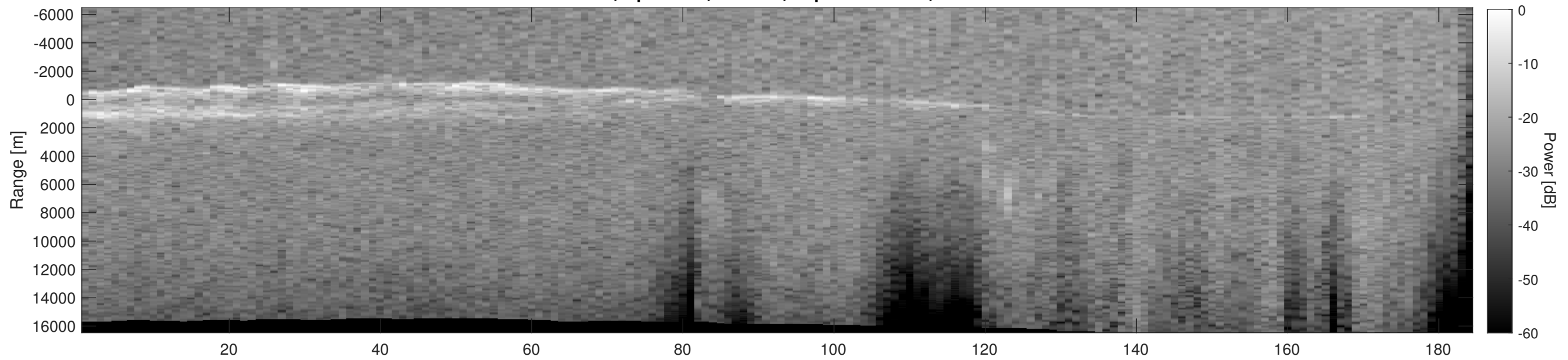
Orbit 5840, Depth-Corrected Cluttergram
