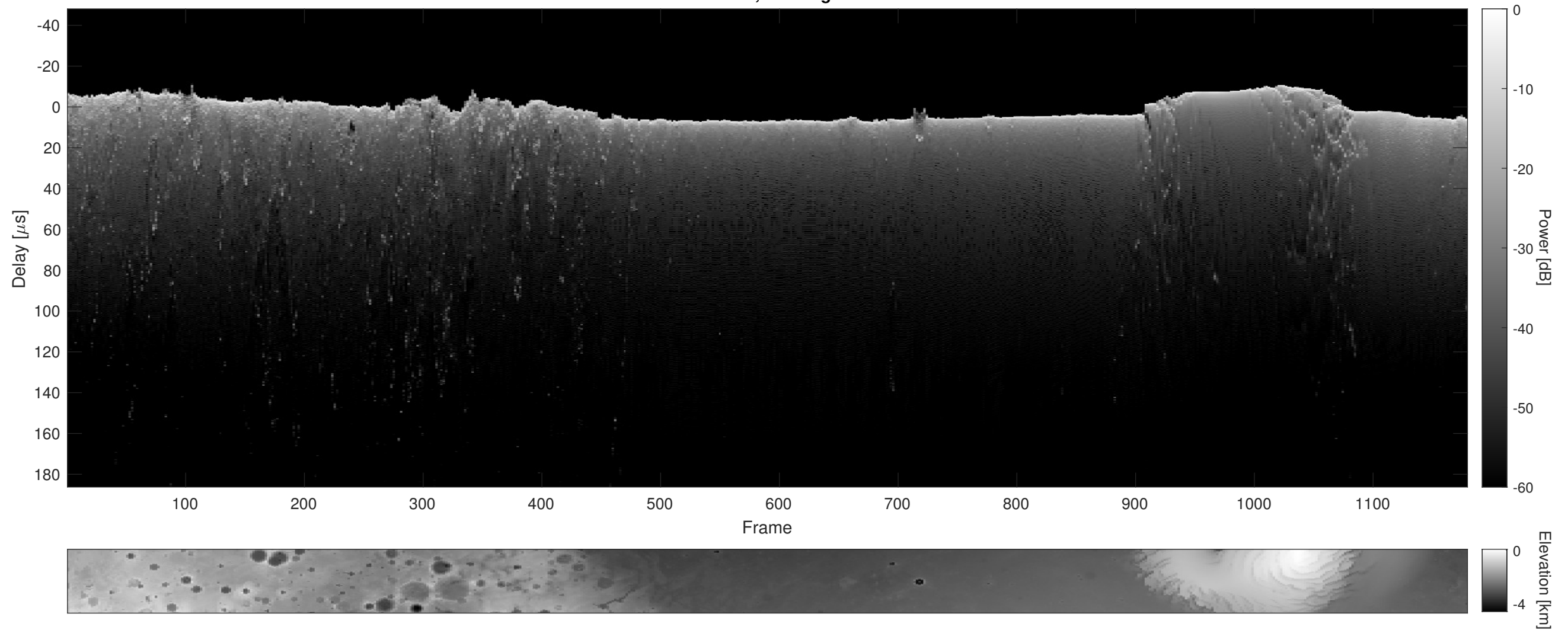
Orbit 5841, Cluttergram
