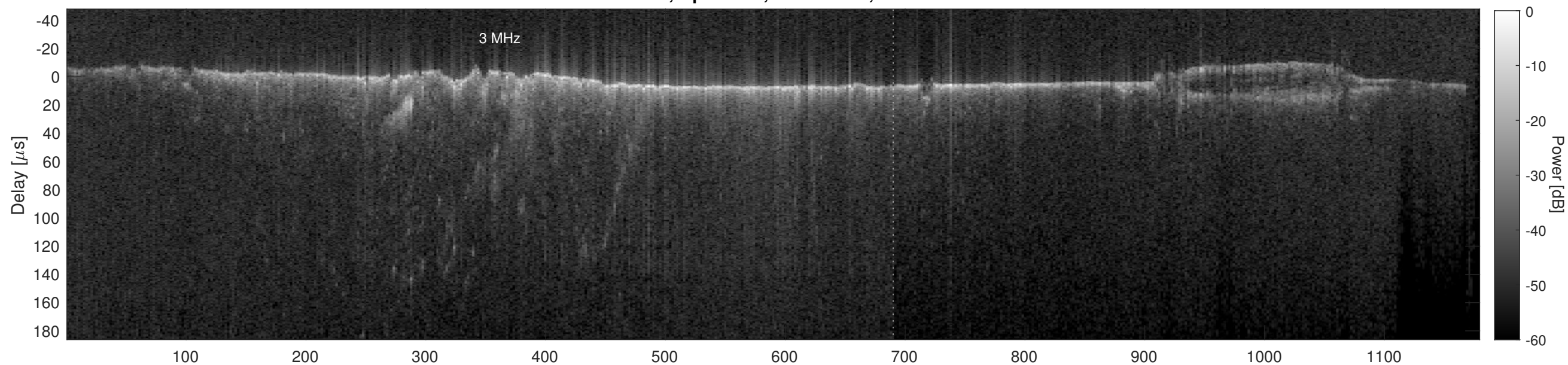
Orbit 5841, Cluttergram
