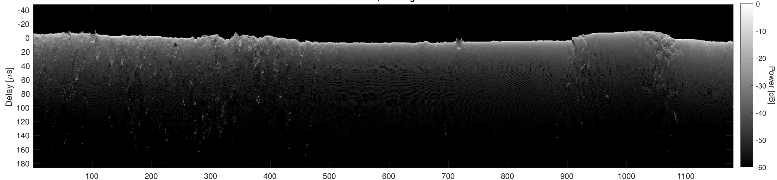
Orbit 5841, Cluttergram
