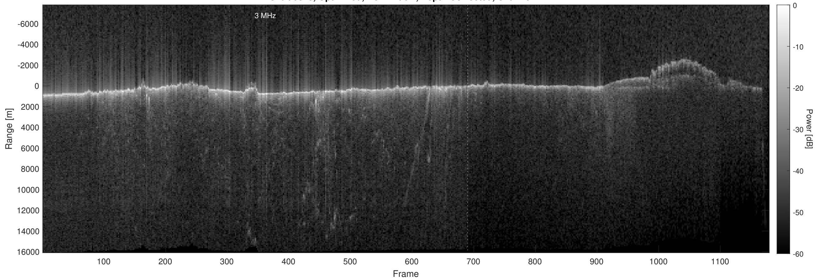
Orbit 5843, Optimized, No Window, Depth-Corrected, Channel 2
