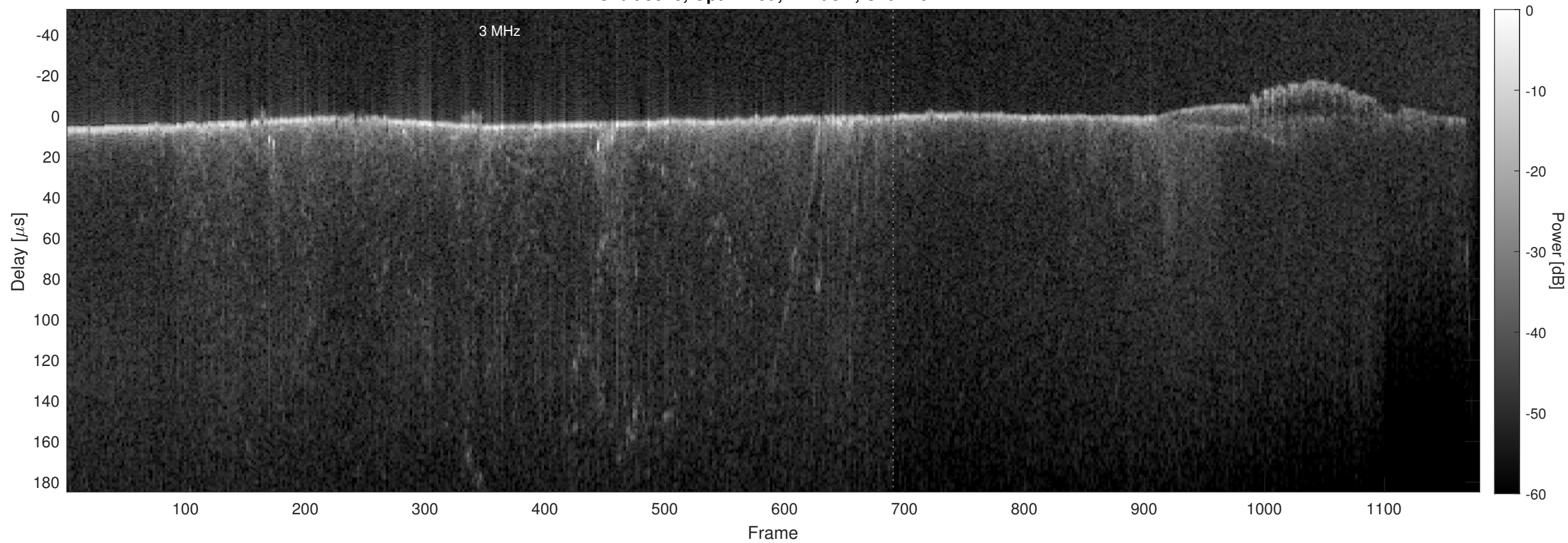
Orbit 5843, Optimized, Window, Channel 2
