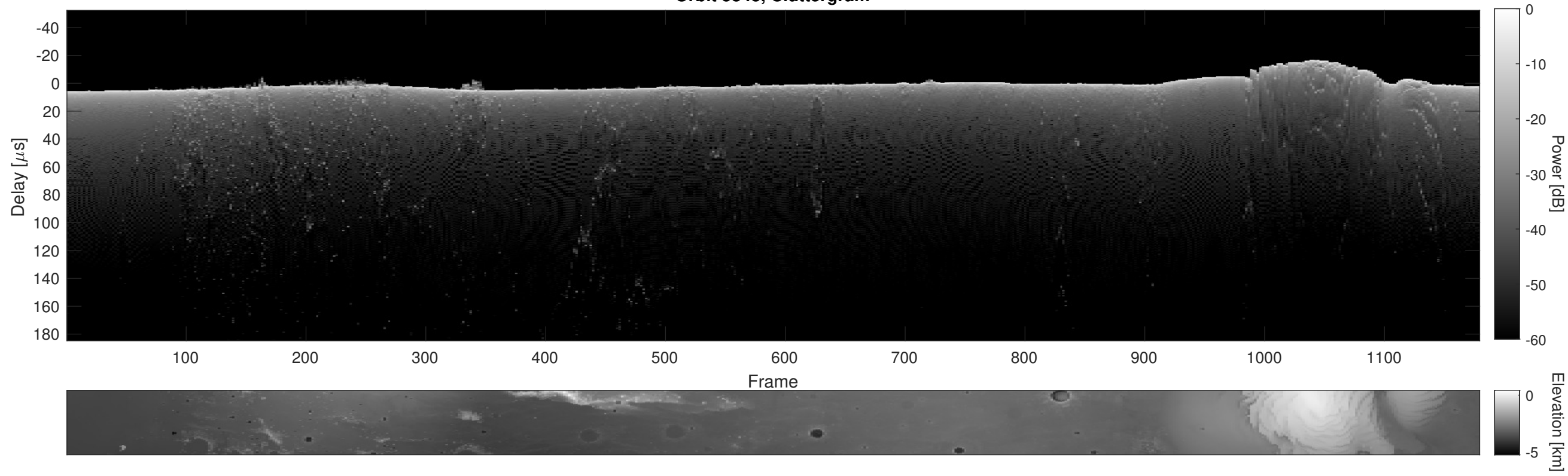
Orbit 5843, Cluttergram
