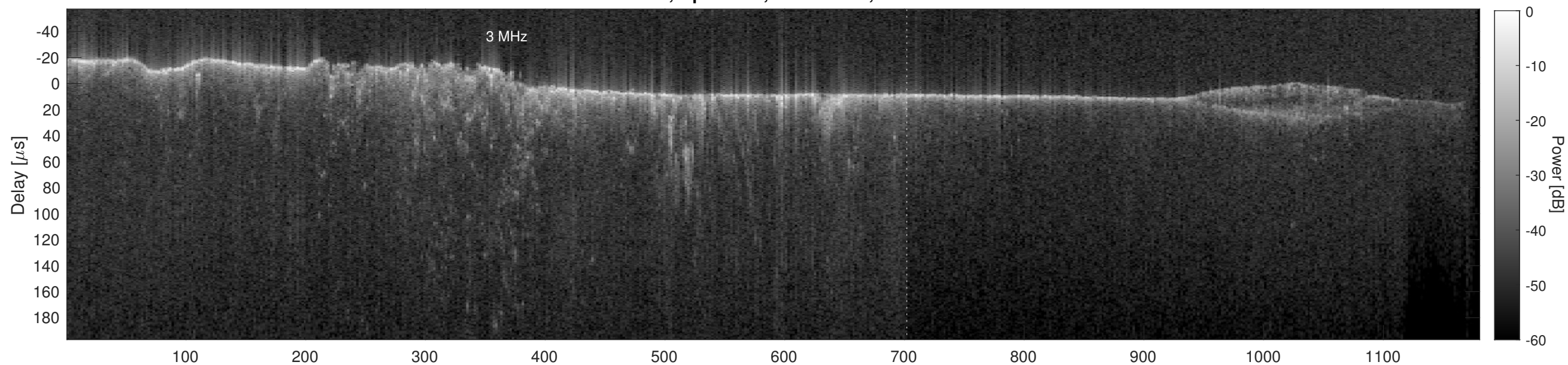
Orbit 5844, Cluttergram
