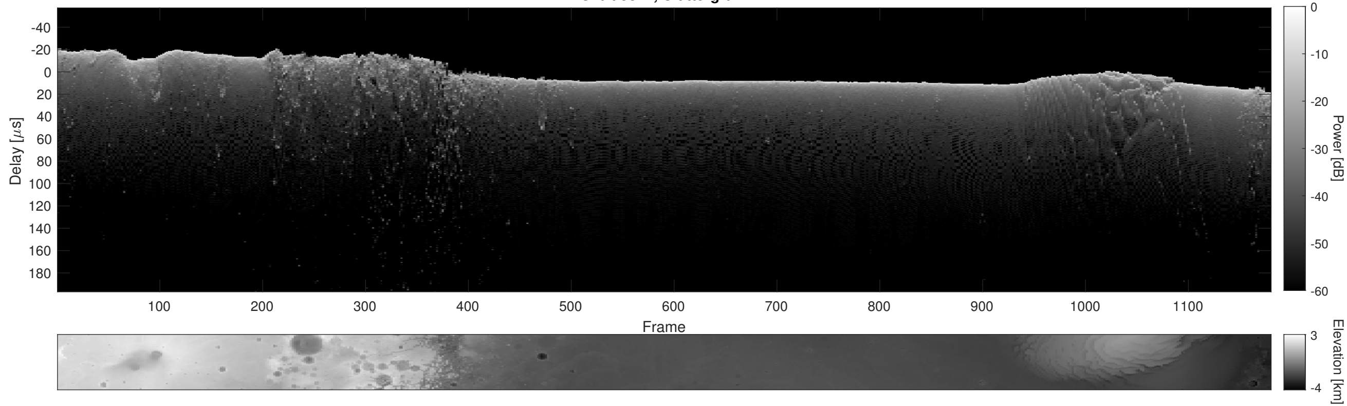
Orbit 5844, Cluttergram
