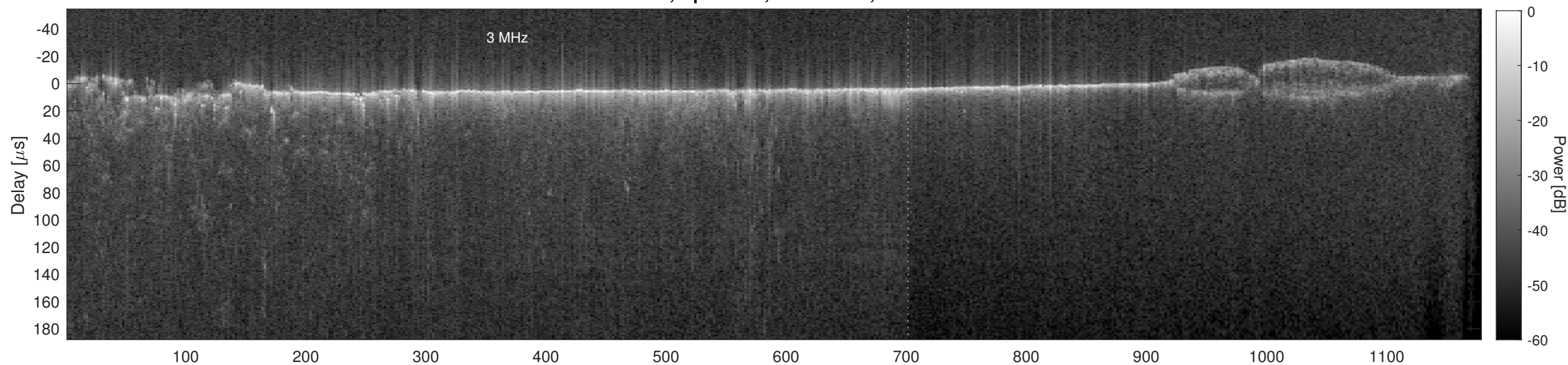
Orbit 5845, Cluttergram
