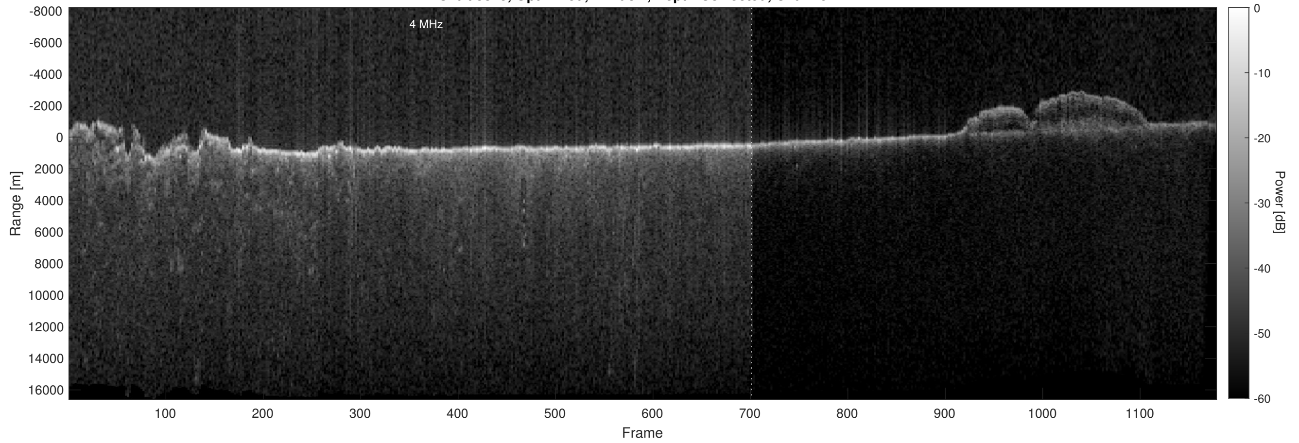
Orbit 5845, Optimized, Window, Depth-Corrected, Channel 2
