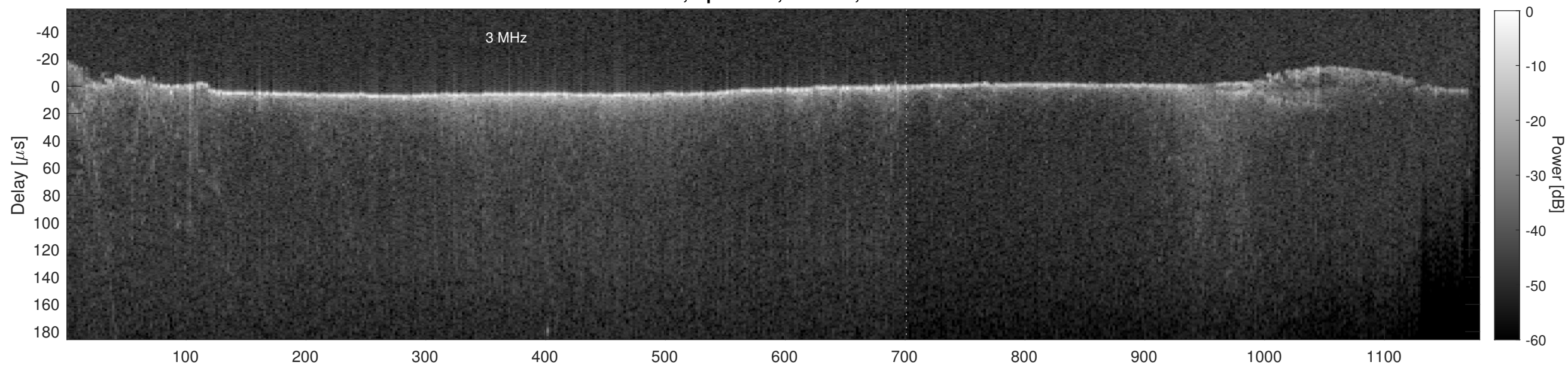
Orbit 5847, Cluttergram
