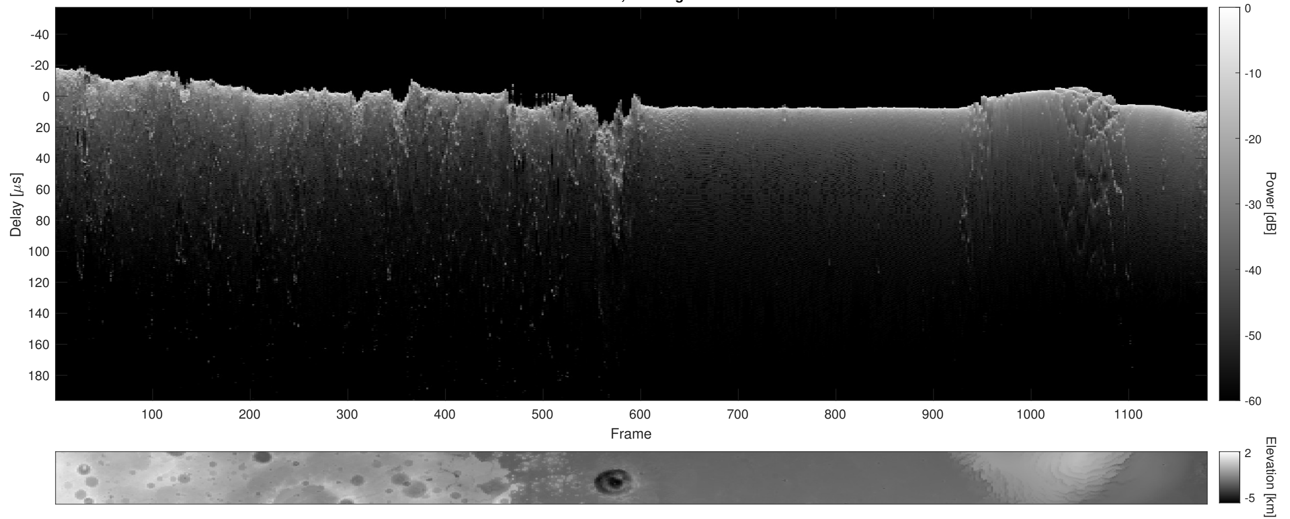
Orbit 5848, Cluttergram
