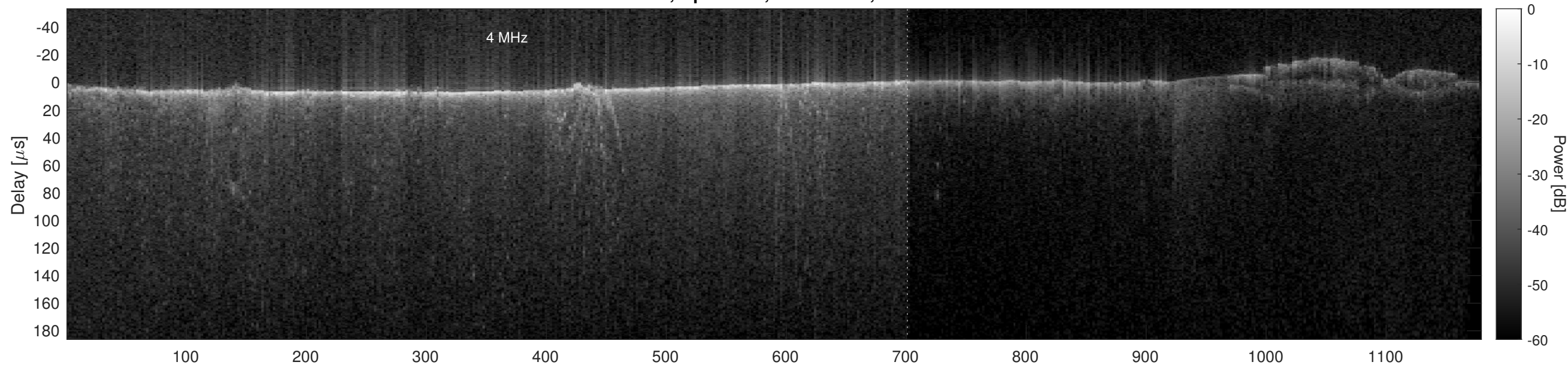
Orbit 5850, Optimized, No Window, Channel 2
