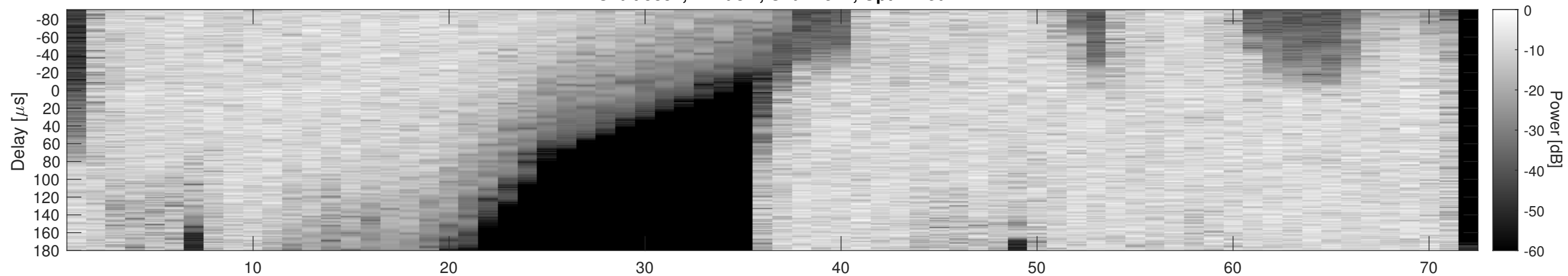
Orbit 5851, Cluttergram
