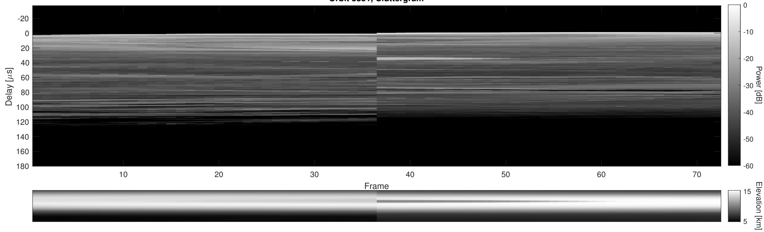
Orbit 5851, Cluttergram
