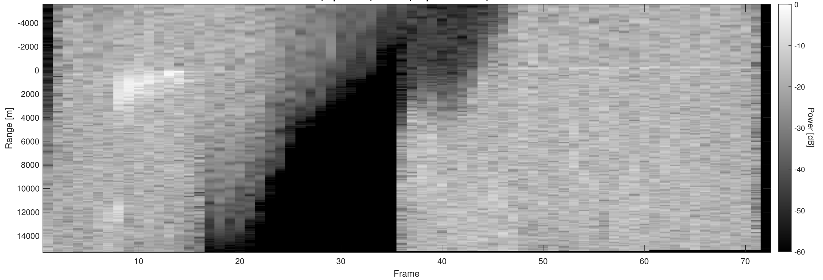
Orbit 5851, Optimized, Window, Depth-Corrected, Channel 2
