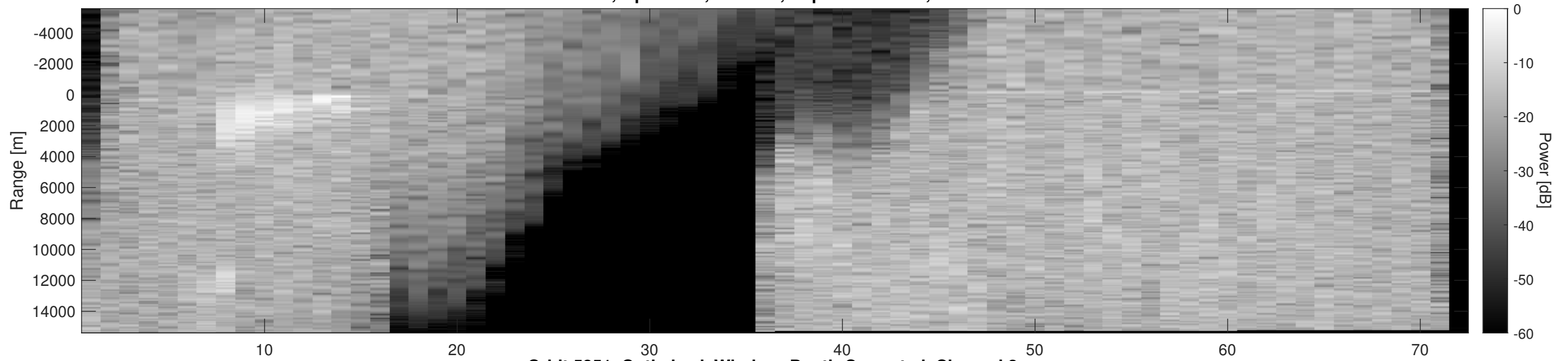
Orbit 5851, Optimized, Window, Depth-Corrected, Channel 2
