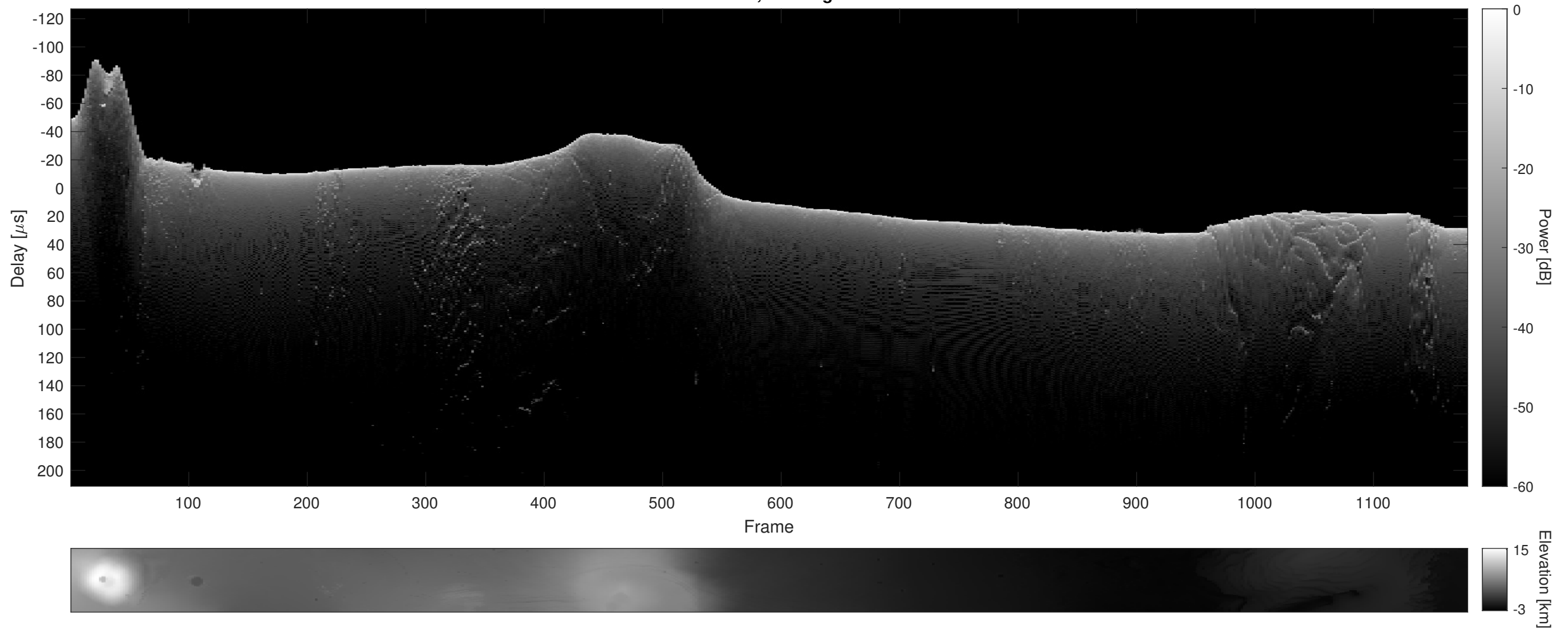
Orbit 5853, Cluttergram
