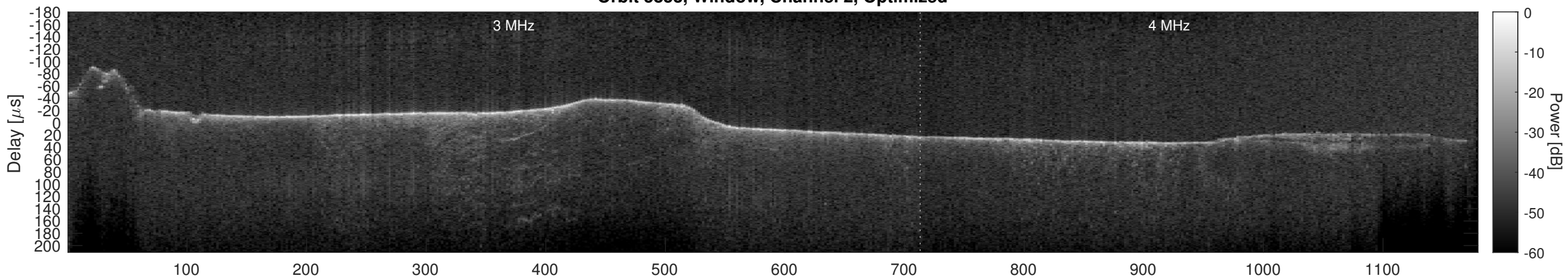
Orbit 5853, Cluttergram
