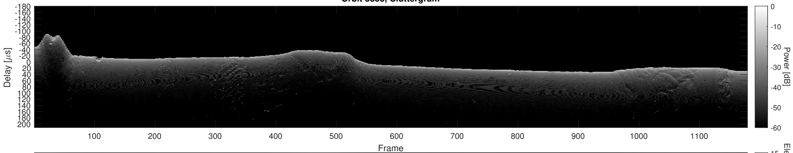
Orbit 5853, Cluttergram
