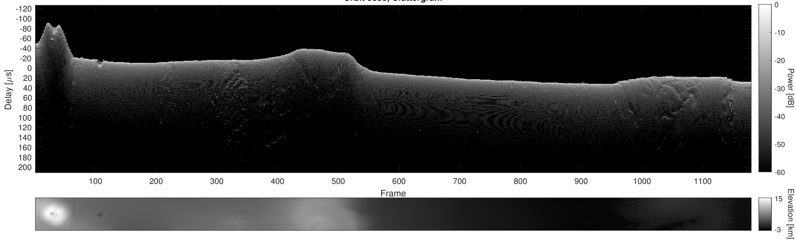
Orbit 5853, Cluttergram
