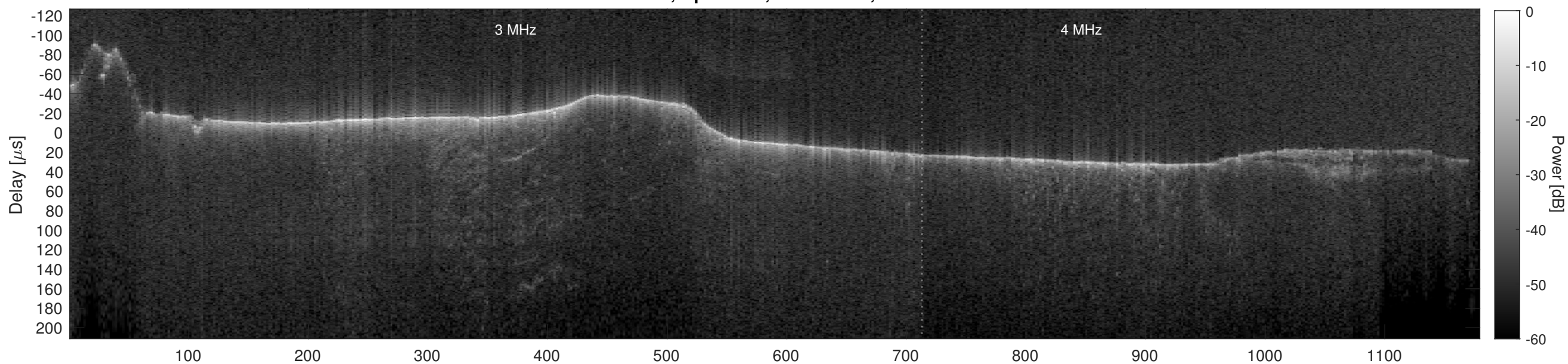
Orbit 5853, Cluttergram
