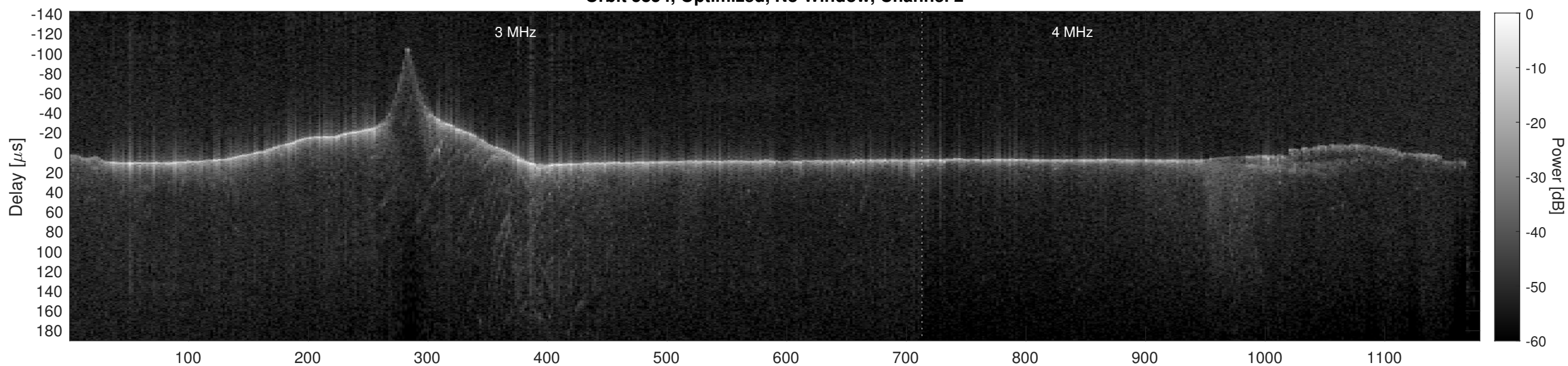
Orbit 5854, Cluttergram
