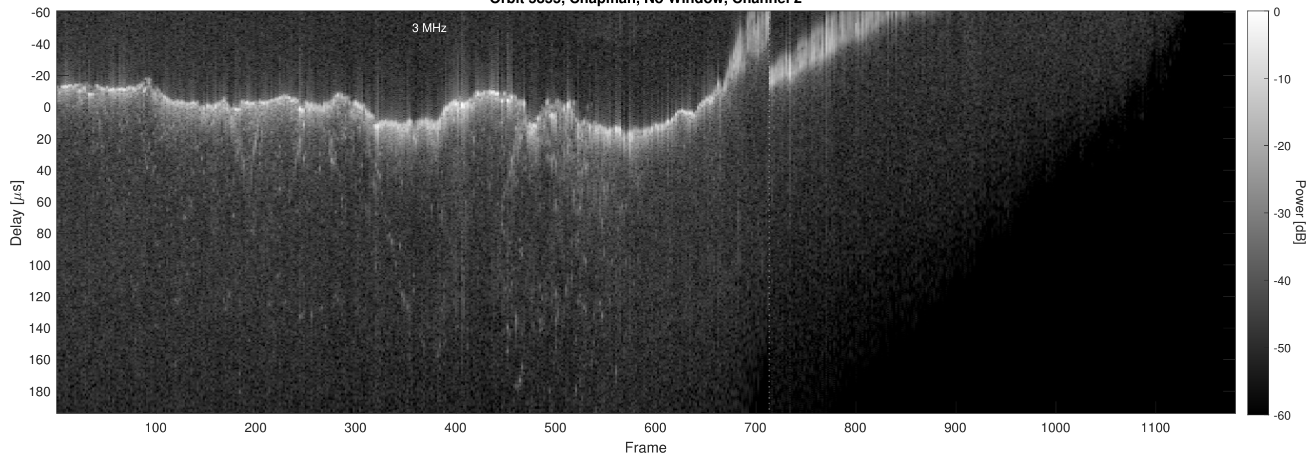
Orbit 5855, Chapman, No Window, Channel 2
