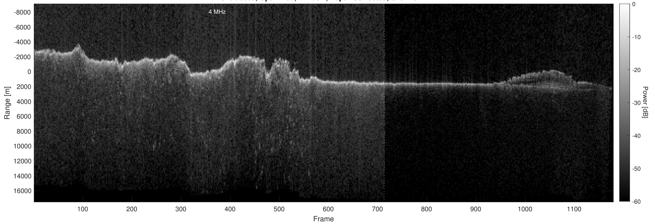
Orbit 5855, Optimized, Window, Depth-Corrected, Channel 2
