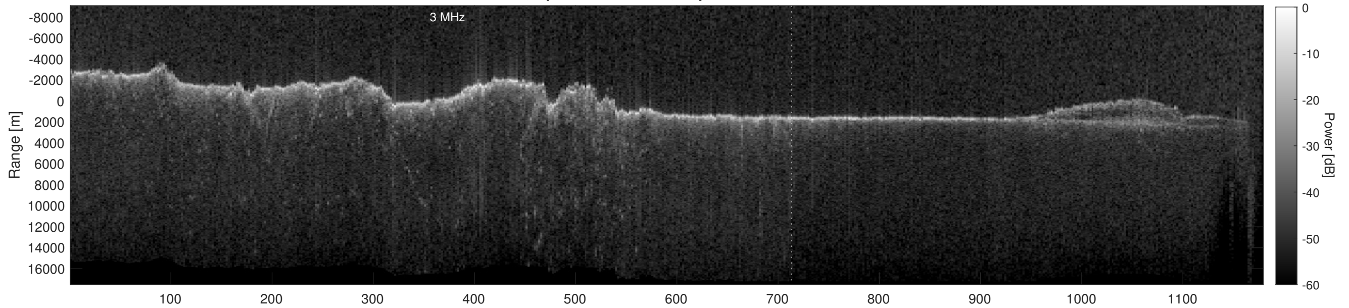
Orbit 5855, Depth-Corrected Cluttergram
