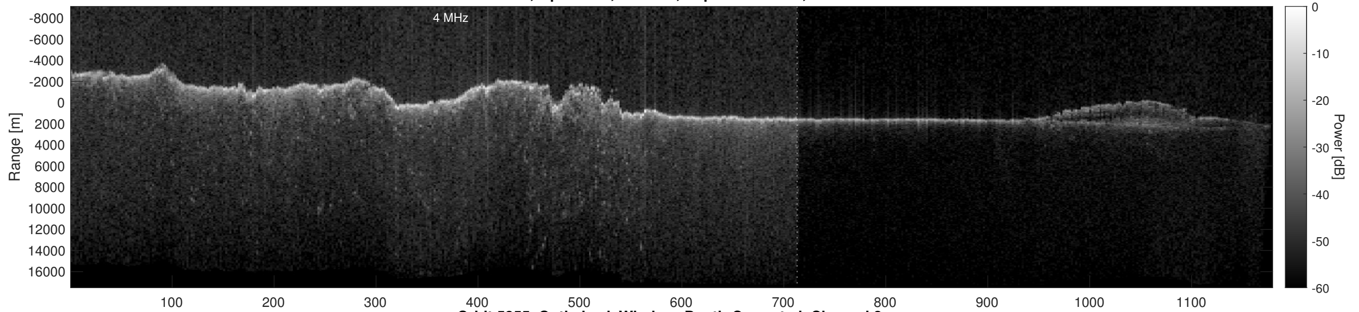
Orbit 5855, Optimized, Window, Depth-Corrected, Channel 2
