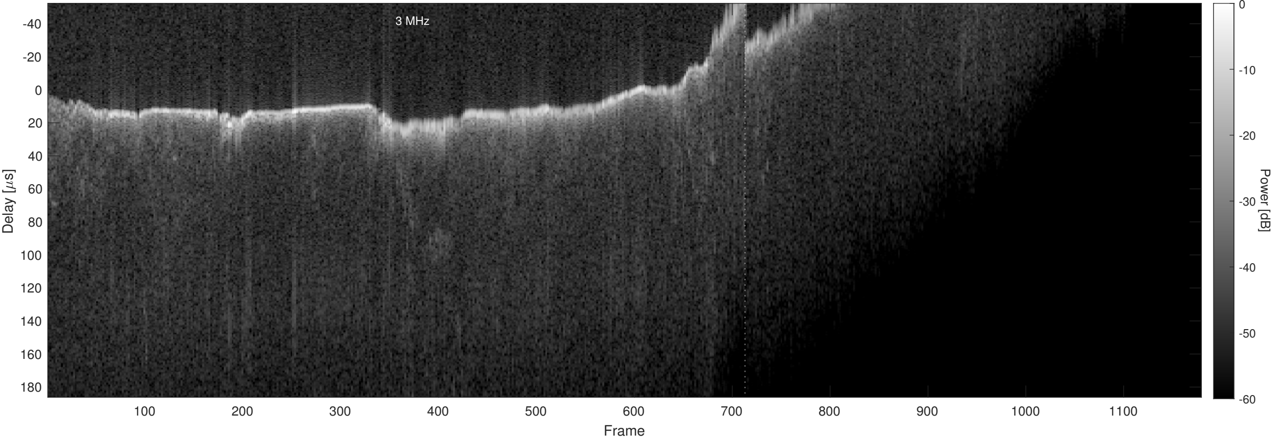
Orbit 5857, Chapman, Window, Channel 2
