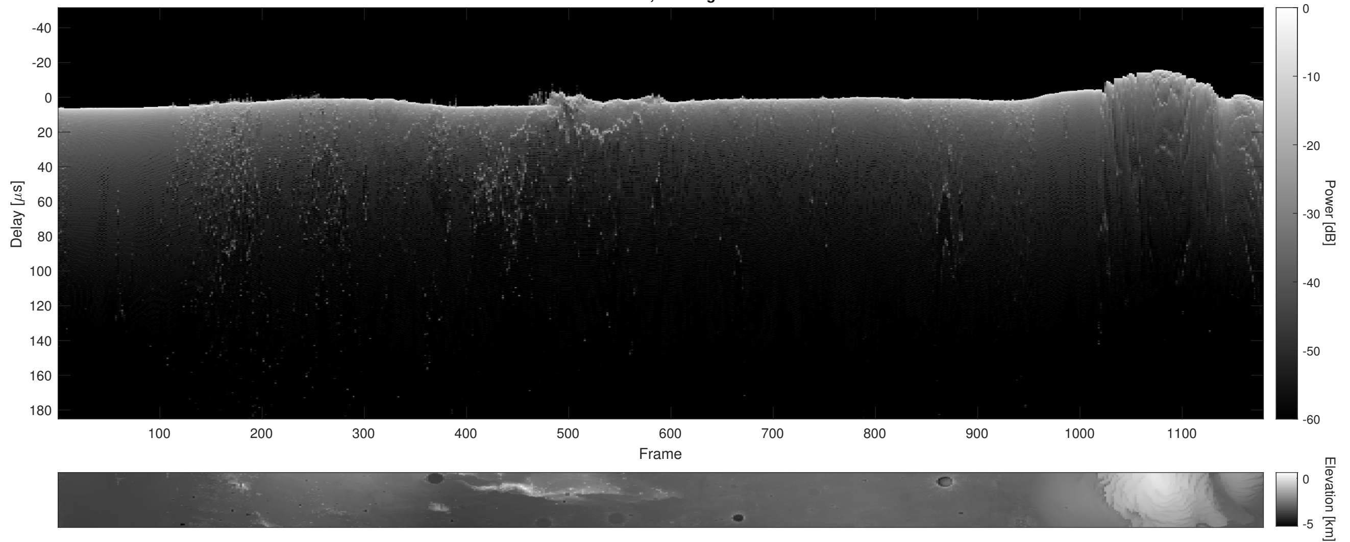
Orbit 5861, Cluttergram
