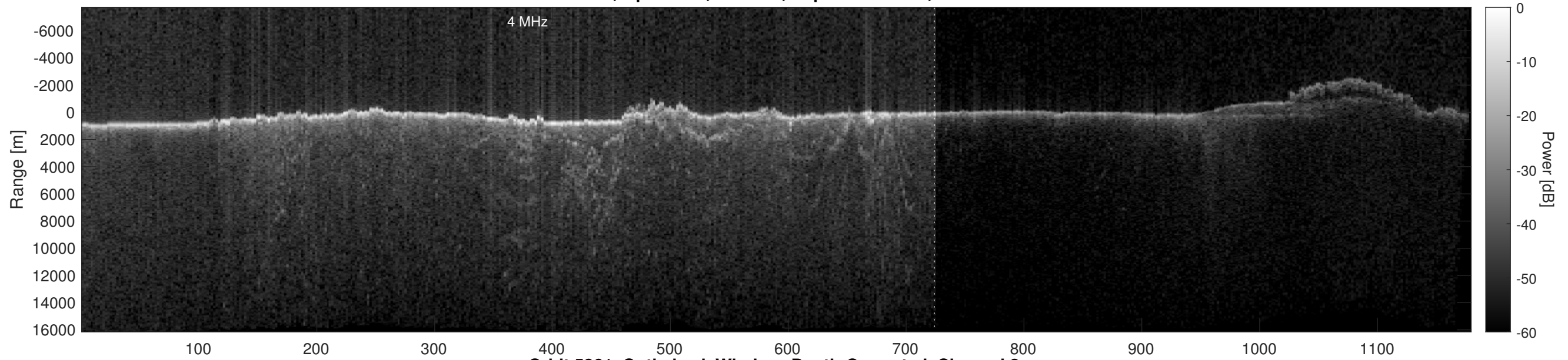
Orbit 5861, Optimized, Window, Depth-Corrected, Channel 2
