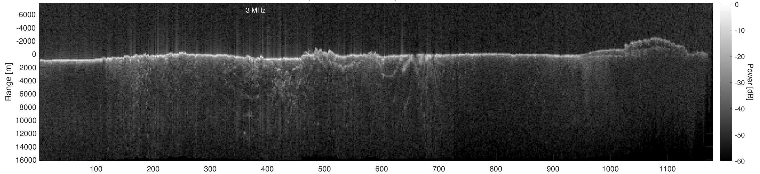
Orbit 5861, Depth-Corrected Cluttergram
