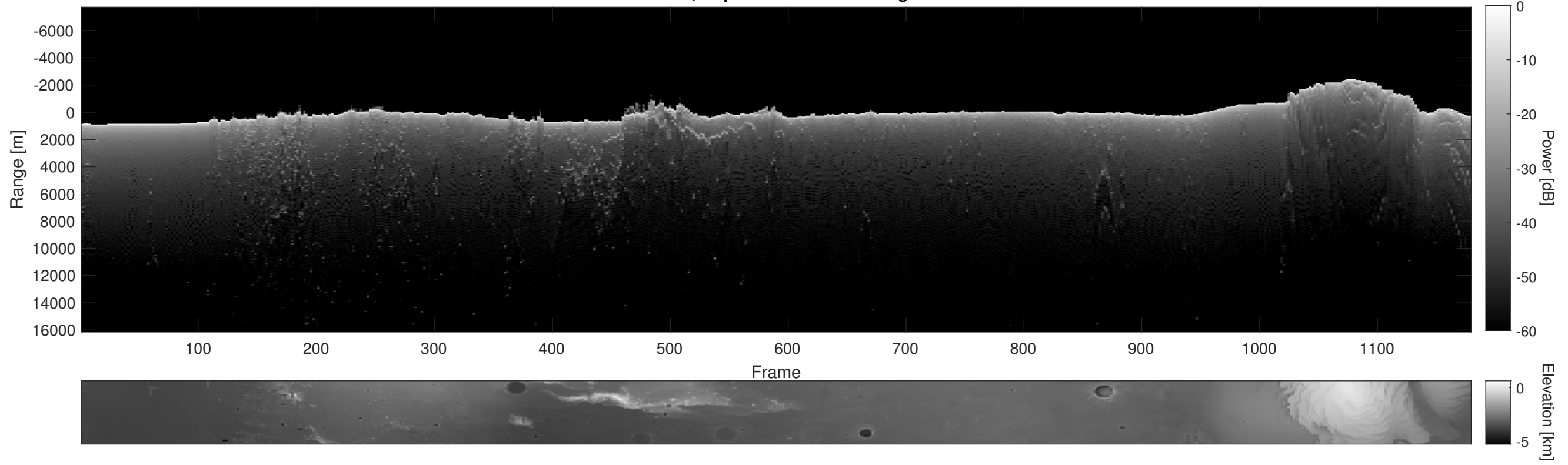
Orbit 5861, Depth-Corrected Cluttergram
