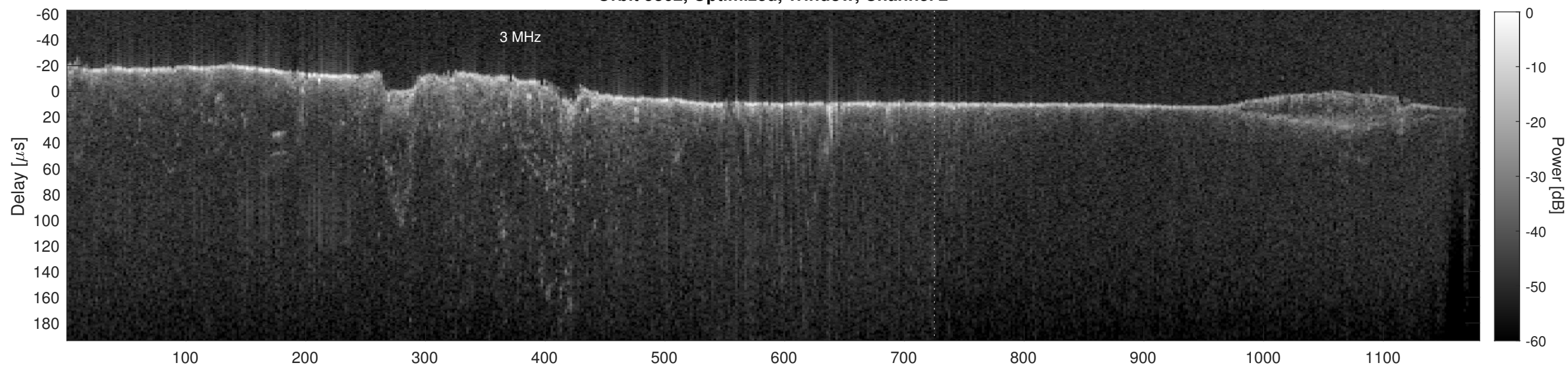
Orbit 5862, Cluttergram
