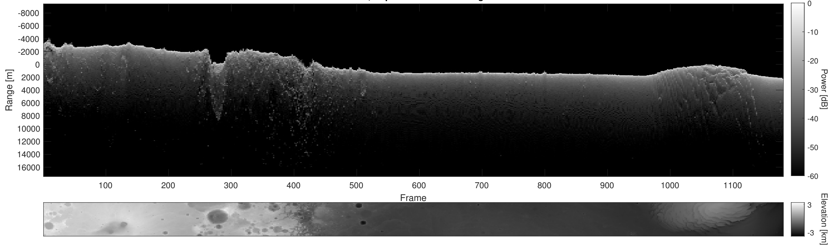
Orbit 5862, Depth-Corrected Cluttergram
