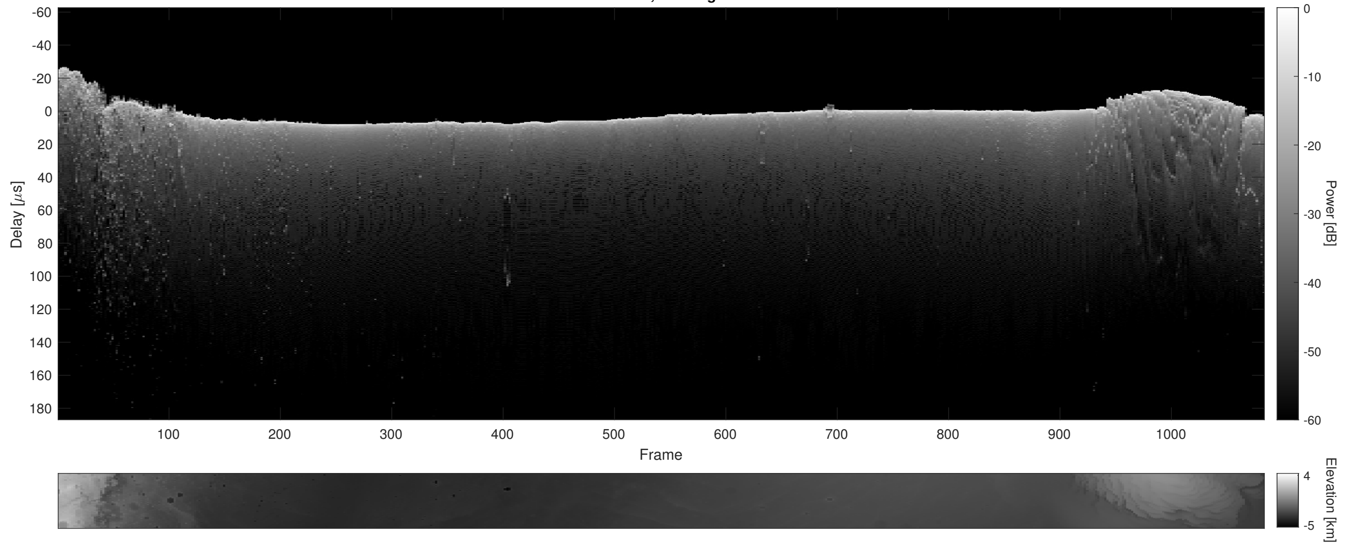
Orbit 5865, Cluttergram
