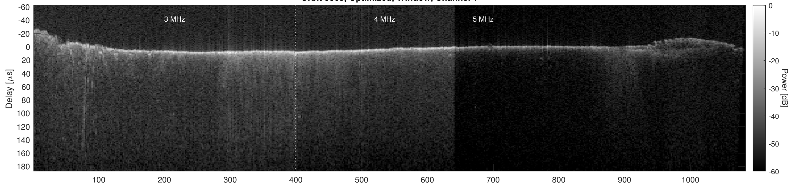
Orbit 5865, Optimized, Window, Channel 2
