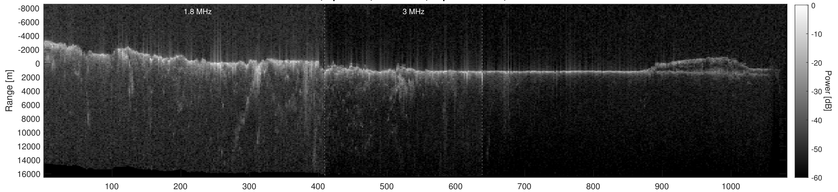
Orbit 5866, Depth-Corrected Cluttergram
