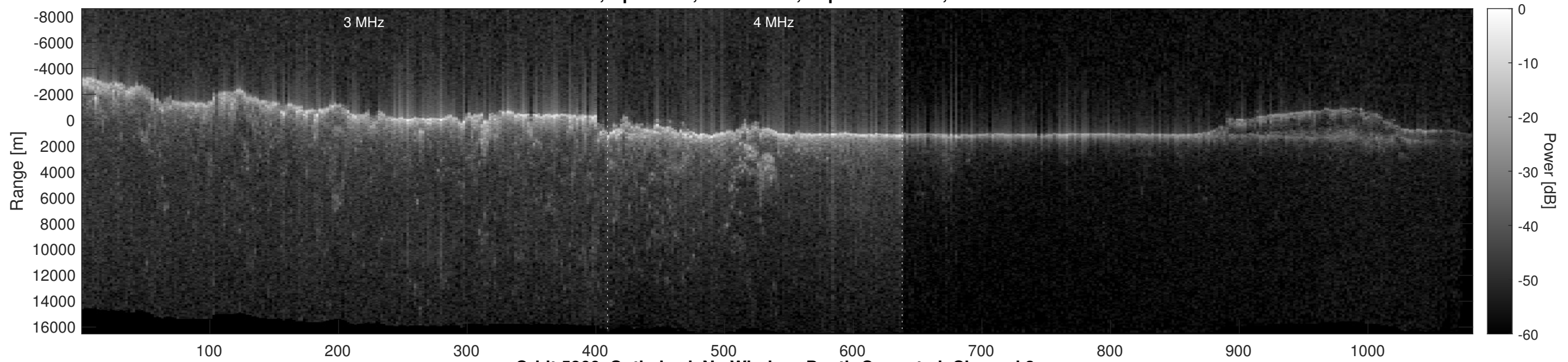
Orbit 5866, Optimized, No Window, Depth-Corrected, Channel 2
