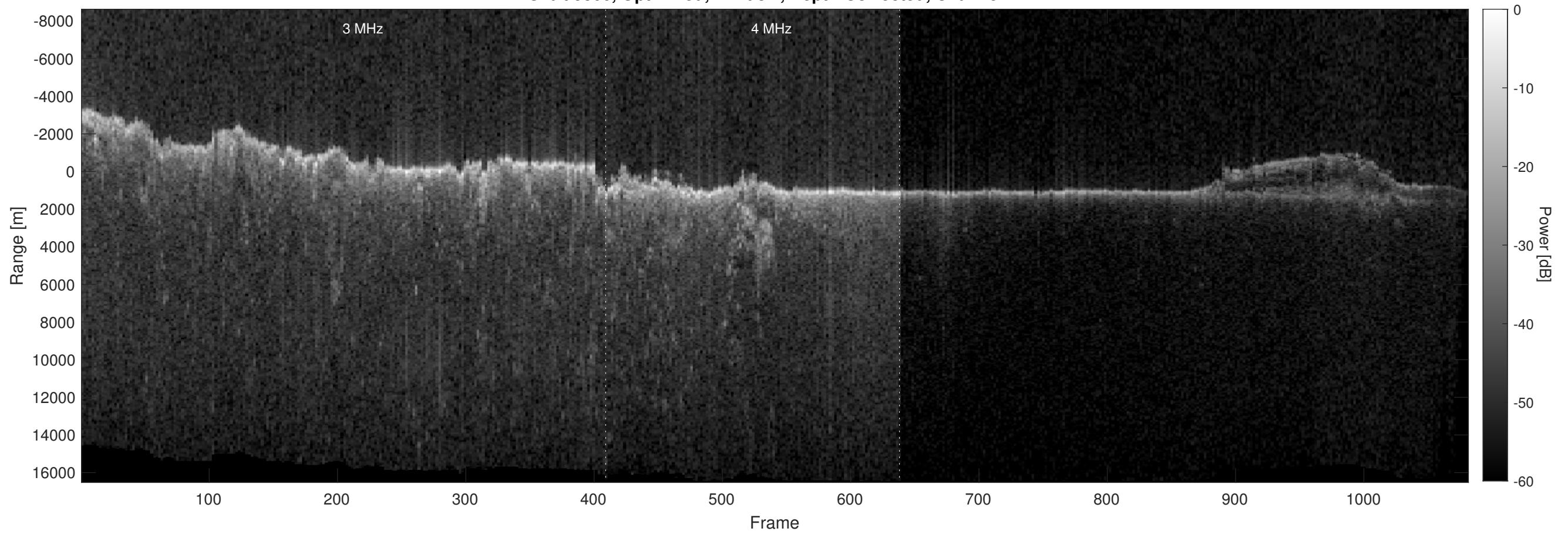
Orbit 5866, Optimized, Window, Depth-Corrected, Channel 2
